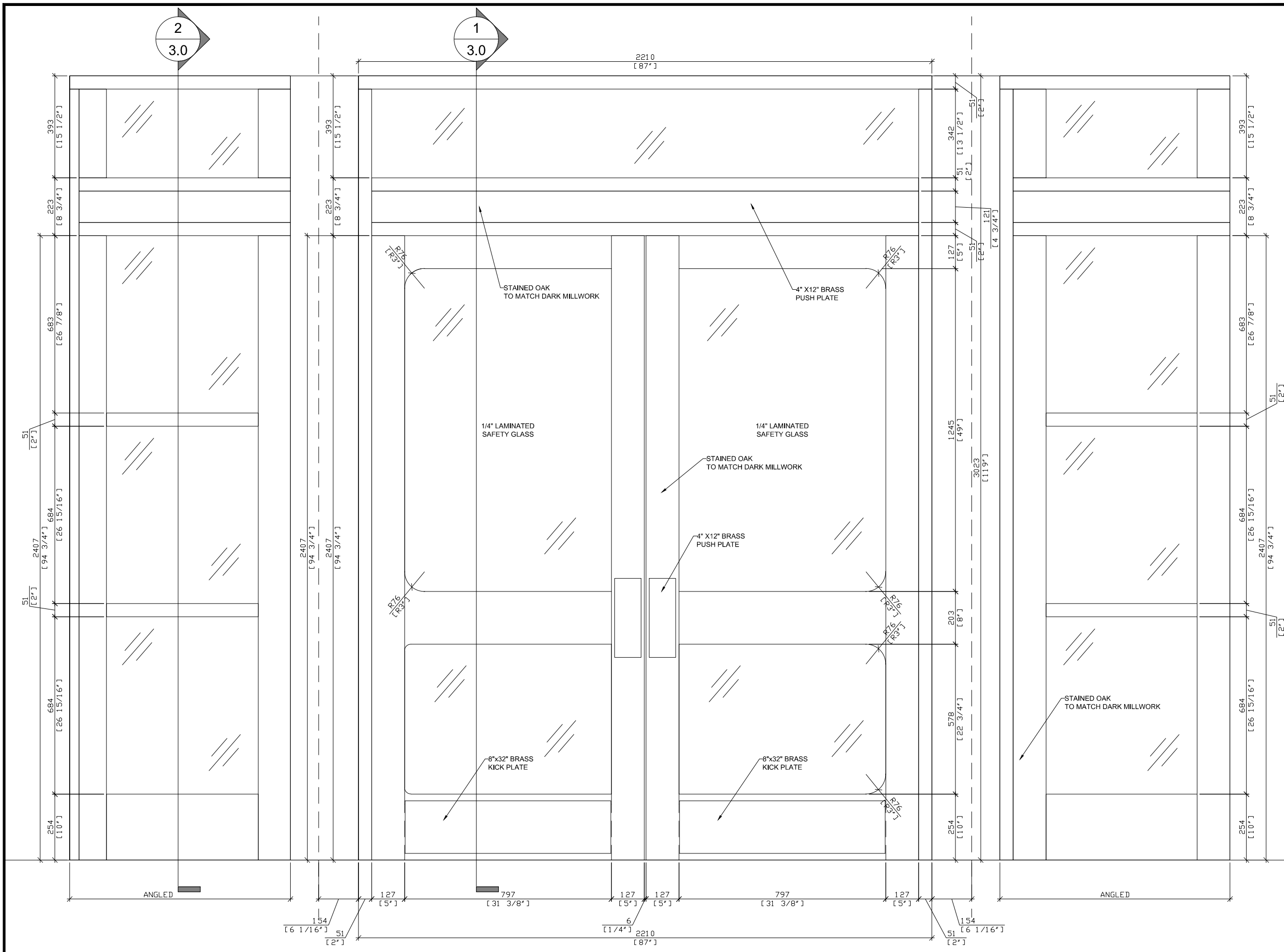
1 2.0 ELEVATION SCALE - 1:10
