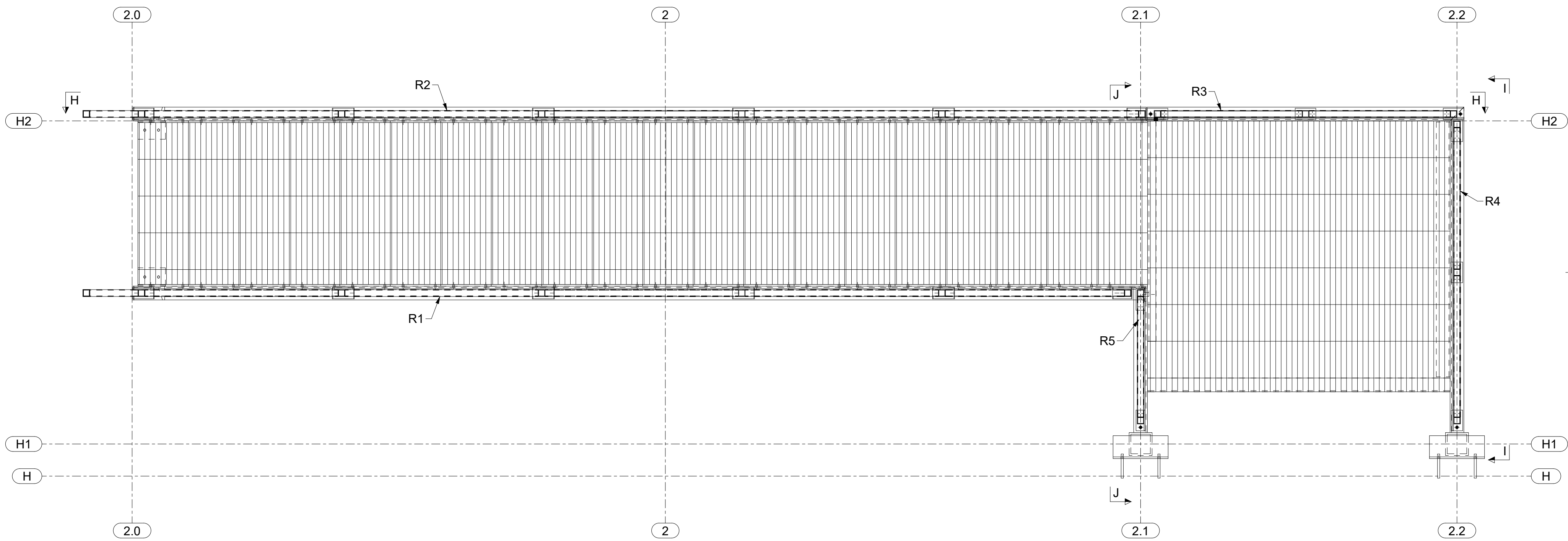
GRATING & HANDRAIL PLAN SCALE: 3/4" = 1'-0"
